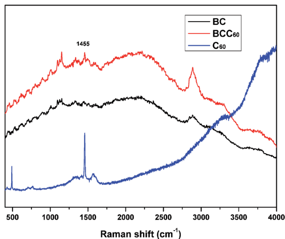
Fig. 2 Raman spectra of the BC, C 60 and BCC 60 composites.
