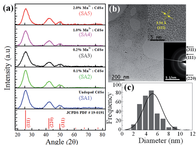
Fig. 3 (a) Powder XRD spectrum of CdSe QDs with different Mn 2+ concentrations along with standard JCPDS file number 19-0191 lines for bulk CdSe. (b) TEM image of 2% Mn 2+ doped CdSe QDs (SA5). Inset (top right) shows the HR-TEM image of a CdSe nanoparticle with well-defined lattice planes of d spacing 3.54 Å. Inset (bottom right) shows SAED pattern of the same sample for crystal planes (111), (220), and (311). (c) Histogram profile of CdSe QDs size derived from (b).
