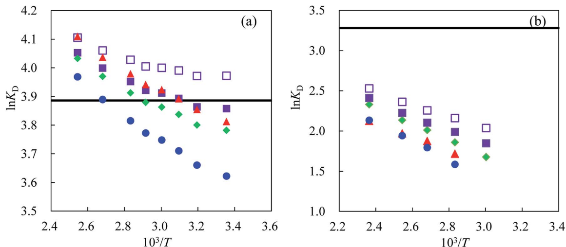
Fig. 6 Plots of \ln K_D for alkali metal ions as a function of reciprocal of temperature on a MCI GEL CK02A column (a) and a Nafion column (b). Eluent: 50 mM TMABr. Symbols: ( \blacktriangle ) \text{Li}^+ , ( \bullet ) \text{Na}^+ , ( \blacklozenge ) \text{K}^+ , ( \blacksquare ) \text{Rb}^+ , ( \square ) \text{Cs}^+ . The solid line denotes the \ln K_D(E) value for each column.
