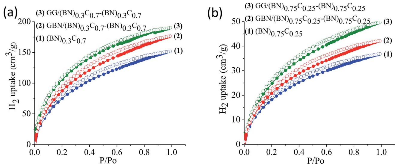
Fig. 11 H 2 adsorption profiles of (a) (BN) 0.3 C 0.7 (1), GBN/(BN) 0.3 C 0.7 –(BN) 0.3 C 0.7 (2), GG/(BN) 0.3 C 0.7 –(BN) 0.3 C 0.7 (3); (b) (BN) 0.75 C 0.25 (1), GBN/(BN) 0.75 C 0.25 –(BN) 0.75 C 0.25 (2), GG/(BN) 0.75 C 0.25 –(BN) 0.75 C 0.25 (3) at 77 K.
