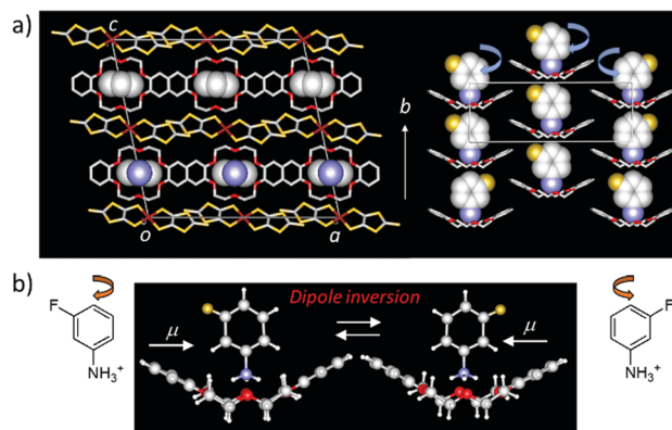
Fig. 9 Two-fold flip-flop motion of m - \text{FAni}^+ cations along the \text{C}-\text{NH}_3^+ axis in monovalent [\text{Ni}(\text{dmit})_2] crystals. (a) Unit cell and supramolecular rotator layer in m - \text{FAni}^+(\text{dibenzo}[18]\text{crown-6})[\text{Ni}(\text{dmit})_2] crystals. (b) The motional freedom of polar m - \text{FAni}^+ cations is sensitive to the dielectric response and resulted in the phase transition from the low temperature ferroelectric to the high temperature paraelectric states.
