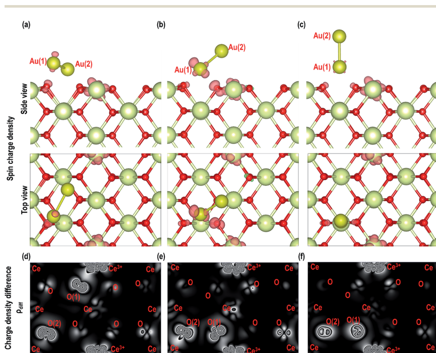
Fig. 12 Top and side view of isosurface ( 0.007 \text{ e } \text{\AA}^{-3} ) of spin densities of \text{Au}_2 on \text{CeO}_2 (110) surface for (a) M_{\text{Au-Dim}} 1, (b) M_{\text{Au-Dim}} 2 and (c) M_{\text{Au-Dim}} 3 and 2D charge density difference contour maps of (d) M_{\text{Au-Dim}} 1, (e) M_{\text{Au-Dim}} 2 and (f) M_{\text{Au-Dim}} 3.
