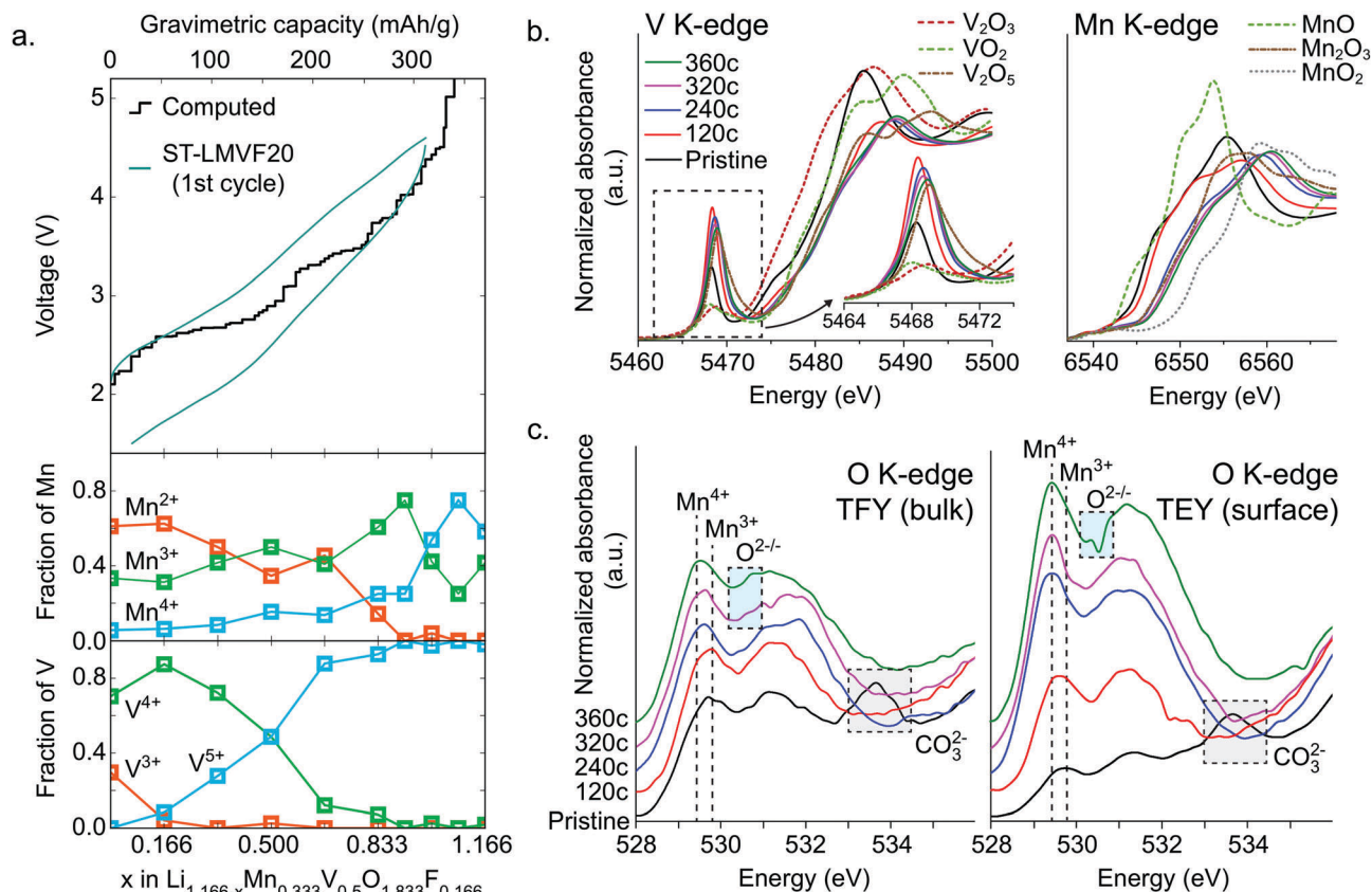
Fig. 4 Oxidation mechanism for the stoichiometric Li 1.171 Mn 0.343 V 0.486 O 1.8 F 0.2 (ST-LMVF20) compound. (a) Computed voltage profile and evolution of Mn and V oxidation states computed from DFT, denoting the dominant source of electron capacity at each stage of delithiation, where we use Li 1.166 Mn 0.333 V 0.5 O 1.833 F 0.166 as a representative composition for ST-LMVF20. (b) XANES at the V and Mn K-edge and (c) soft XAS at the O K-edge for ST-LMVF20 at various states of charge within the first cycle.
