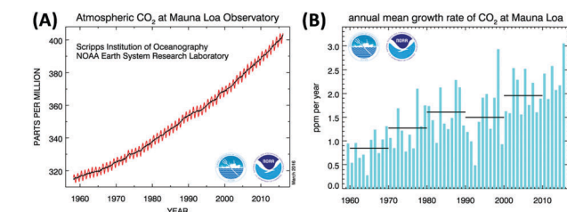
Fig. 1 (A) Increase of the atmospheric CO 2 concentration measured during 1958–2015 at the Mauna Loa (Hawaii). The red curve shows seasonal fluctuations, the black curve represents seasonally corrected data. (B) Annual mean carbon dioxide concentration growth rates. Decadal averages of the growth rate are also plotted as horizontal black lines. 6
