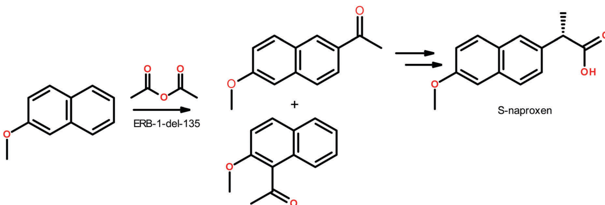
Scheme 4 Acylation of 2-methoxynaphthalene with acetic anhydride and illustration of the route to S-naproxen.
