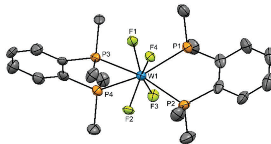
Fig. 1 The cation present in [WF 4 {o-C 6 H 4 (PME 2 ) 2 } 2 ][WOF 5 ] 2 ·MeCN showing the atom numbering scheme and with ellipsoids drawn at the 50% probability level. H atoms are omitted for clarity. Selected bond lengths (Å) and angles (°): W(1)–F(3) = 1.91(4), W(1)–F(2) = 1.92(4), W(1)–F(1) = 1.92(4), W(1)–F(4) = 1.93(4), W(1)–P(3) = 2.572(17), W(1)–P(1) = 2.579(18), W(1)–P(2) = 2.582(18), W(1)–P(4) = 2.592(18), P(3)–W(1)–P(4) = 72.6(6), P(1)–W(1)–P(2) = 72.8(6).
