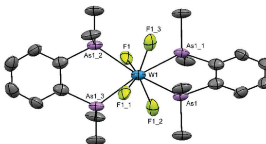
Fig. 2 The cation present in [\text{W}_4\text{I}_6\text{-C}_6\text{H}_4(\text{AsMe}_2)_2]_2[\text{W}_8] showing the atom numbering scheme and with ellipsoids drawn at the 50% probability level. Hydrogen atoms are omitted for clarity. Selected bond lengths (Å) and angles (°): \text{W}(1)\text{-F}(1) = 2.114(6) , \text{W}(1)\text{-As}(1) = 2.6279(10) , \text{As}(1)\text{-W}(1)\text{-As}(1) \#1 = 75.74(4) . Symmetry operators: \#1 = -x + 5/4, -y + 5/4, z ; \#2 = x, -y + 5/4, -z + 1/4 ; \#3 = -x + 5/4, y, -z + 1/4 .
