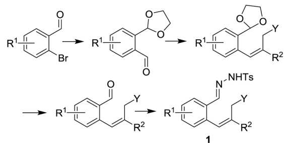
Horner-Wadsworth-Emmons approach
