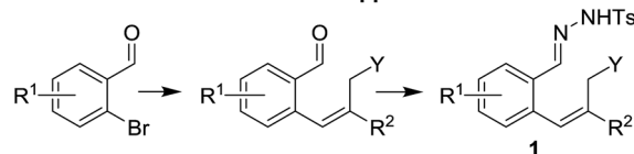
Heck-coupling approach
