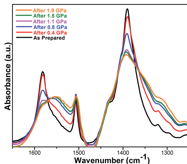
Fig. 3 FT-IR spectra of UiO-66 over the range of 1650–1250 \text{cm}^{-1} after compression and release. All absorbances were normalized to the peak at 1019 \text{cm}^{-1} ( cf. ESI Fig. S4†).
