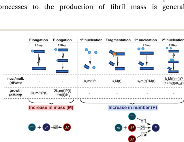
Fig. 3 Processes of fibrillar self-assembly. The processes that make up the reaction network of filamentous self-assembly fall into two categories, nucleation/multiplication processes, which produce new fibril ends, P , and only a negligible quantity of new fibril mass, and growth processes, which produce fibril mass, M , but leave the fibril number unchanged. The contributions to the rates of growth and nucleation/multiplication are given below the schematic representation for each process. For elongation and secondary nucleation we use two alternative schemes, a single-step and a two-step one. Under certain conditions the single-step description may be sufficient, as discussed in the main text. The rate constants and reaction rates are defined in Table 1.
