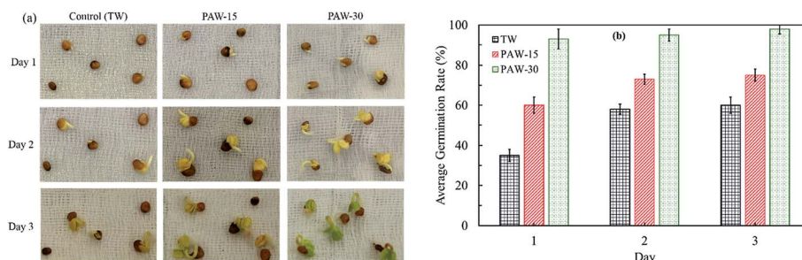
Fig. 4 (a) Seedling growth and (b) average germination rate of radish seeds watered with TW and PAW during the first 3 days after sowing on cotton.
