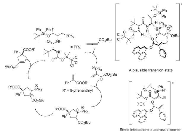
Scheme 23 The proposed mechanism and a key transition state to account for the enantioselectivity.
