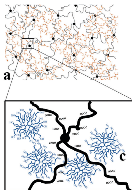
Fig. 10 (a) Interpenetrating networks of PAA-HB; (b) schematic structure of a HB molecule; and (c) schematic illustration of the possible physical interaction and hydrogen bond formation mechanism between PAA chains and HB molecules.
