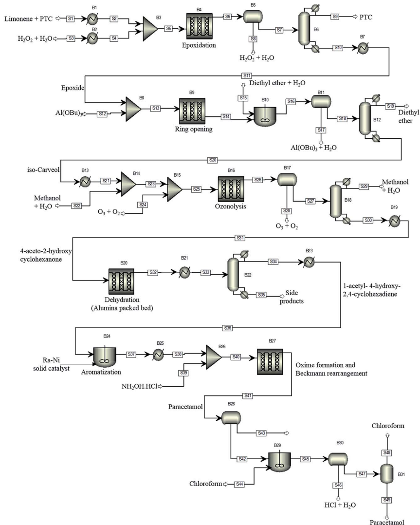
Fig. 4 The proposed process flowsheet detailing all reaction and separation steps. The ASPEN flowsheet is shown for illustration only. All simulations were performed using qPROMS.
