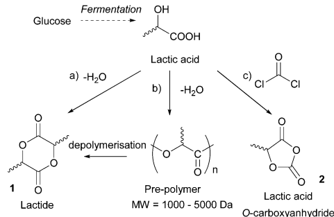
Fig. 2 Routes from LA to lactide via (a) zeolite-catalysed condensation and (b) oligomer depolymerisation ( M_w : molecular weight). (c) Synthesis of lactic acid O -carboxyanhydride from LA.
