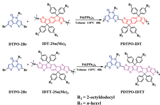
Scheme 1 Synthesis and chemical structures of PDTPB-IDT and PDTPB-IDTT .
