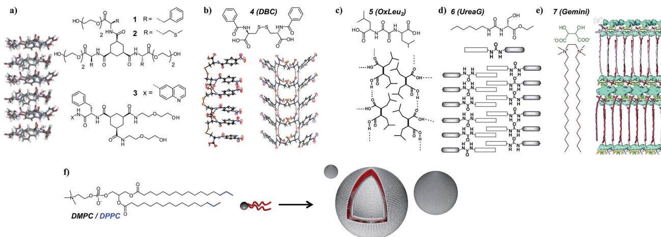
Fig. 2 Various low molecular weight hydrogelators and their expected molecular arrangement in gel fibers: (a) 1,3,5-triamide cis,cis -cyclohexane derivatives 1 , 2 and 3 , (b) dibenzoyl cysteine (DBC), (c) bis(leucine) oxalyl-amide, (d) monourea ethyl serine gelator, and (e) gemini tartrate surfactant. The typical structure of the phosphatidylcholine phospholipids used in this study is also depicted (f). Crystal structures and schemes are reproduced with permission from ref. 39–41.
