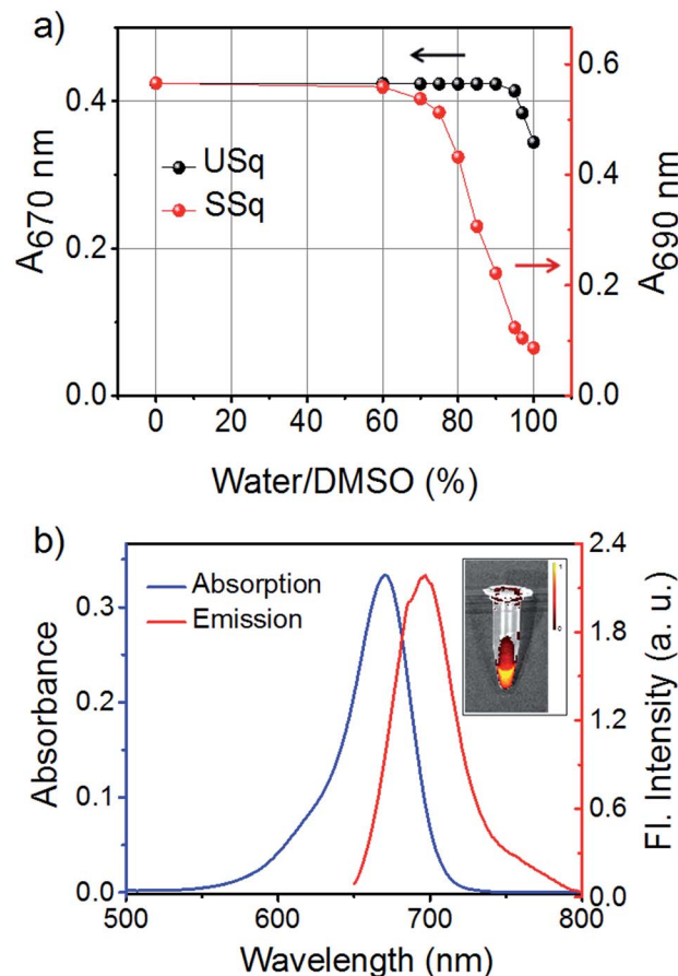
Fig. 1 (a) Changes in the absorption spectra of USq and SSq (2 \mu\text{M} ) in DMSO upon increasing the content of water from 0–100%. (b) UV/Vis absorption (blue curve) and emission spectra (red curve, \lambda_{\text{ex}} = 640\ \text{nm} ) of USq (2 \mu\text{M} ) in 96% phosphate buffer (pH 7.8)/DMSO mixture. Inset shows false-color pixel intensity map image of USq ( \lambda_{\text{ex}} = 640\ \text{nm} ) in 96% phosphate buffer/DMSO mixture.
