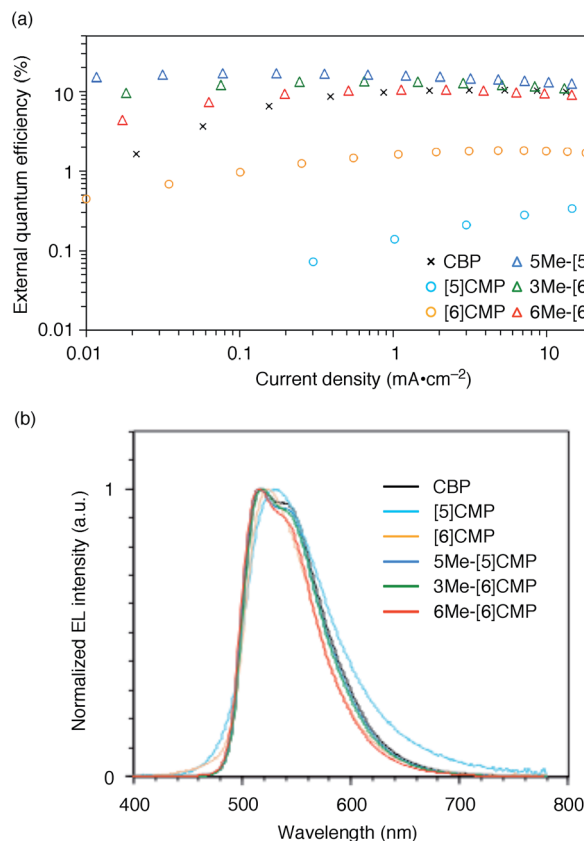
Fig. 2 Performance of the multi-layer OLEDs with various hosts. (a) External quantum efficiency plotted as a function of current density. See Fig. 1a for the device architecture. (b) Electroluminescence spectra at a current density of 0.1 mA cm -2 .
