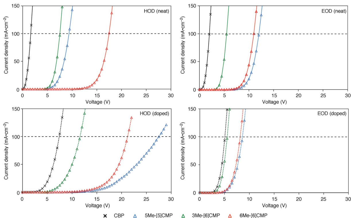
Fig. 7 J - V characteristics of the HOD and EOD are shown for the devices in the absence (neat) or presence (doped) of \text{Ir}(\text{ppy})_3 (6 wt%). The horizontal broken line shows 100 \text{ mA cm}^{-2} . The HOD device was assembled with an ITO (110 nm)/PEDOT:PSS (30 nm)/organic layer (60 nm)/ \alpha -NPD (20 nm)/Al (100 nm) architecture, and the EOD device was assembled with an ITO (110 nm)/PEDOT:PSS (30 nm)/Ca (5 nm)/organic layer (60 nm)/Cs (1.5 nm)/Al (100 nm) architecture. The organic layer was composed either of a single material (neat) or a material containing 6 wt% \text{Ir}(\text{ppy})_3 dopant (doped).
