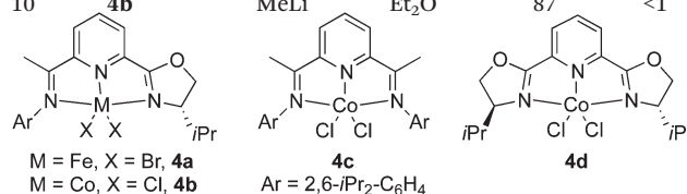
Scheme 1 Transition-metal-catalyzed sequential hydroboration of terminal alkynes.
