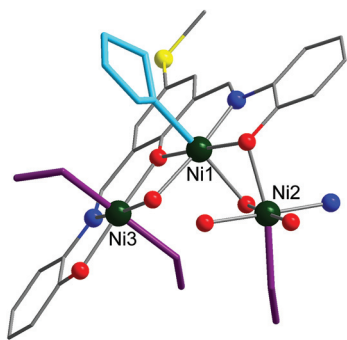
Fig. 3 A fragment of compound 1 representing pseudo-octahedral coordination geometries of the Ni(II) centres. For clarity, only one chelating Schiff-base ligand \text{L-SMe}^{3-} is explicitly depicted. The nickel, nitrogen, oxygen, and sulfur atoms are represented as ball-and-stick models. The terminal-coordinated solvent molecules are highlighted in different colours: MeOH, purple; THF, sky blue. Elemental colour code: C, grey; N, blue; O, red; S, yellow; Ni, dark green.
