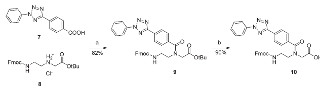
Fig. 4 Synthesis of the tetrazole-containing PNA monomer. (a) \text{HATU} , \text{HOBT} , \text{DIPEA} , \text{DMF} , o.n., RT. (b) \text{DCM}:\text{TFA}:\text{TIPS} 2:1:0.4, o.n., RT.
