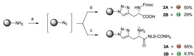
Fig. 3 One-pot click reactions. (a) \text{TfN}_3 , \text{CuSO}_4 , \text{NaHCO}_3 , \text{H}_2\text{O}/\text{MeOH}/\text{DCM} , 30 min, RT. (b) \text{Fmoc-L-Pra-OH} , \text{TBTA} , \text{CuSO}_4 , Na ascorbate, 1 h, MW 80 °C. (c) \text{NLS-Pra} , \text{TBTA} , \text{CuSO}_4 , Na ascorbate, 1 h, MW 80 °C. All amine groups in the peptide sequence are present as TFA salts.
