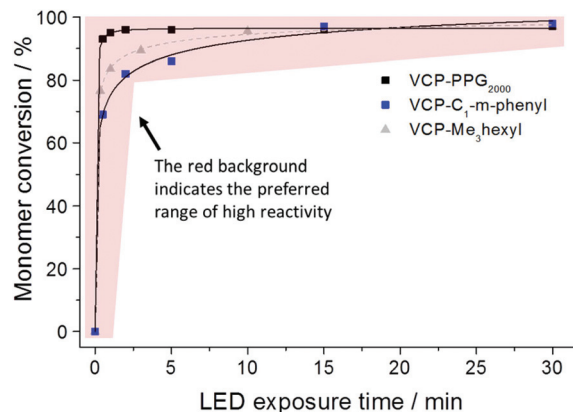
Fig. 3 Determined monomer conversion for the photo-polymerization of VCP-PPG 2000 , VCP- m -phenyl and VCP-Me 3 hexyl (1 mol% initiator CQ: EDMAB in a molar ratio of 1:2). The curing was performed under a controlled atmosphere of nitrogen using a commercial LED source ( 2.013\text{ mW cm}^{-2} for 465 nm).
