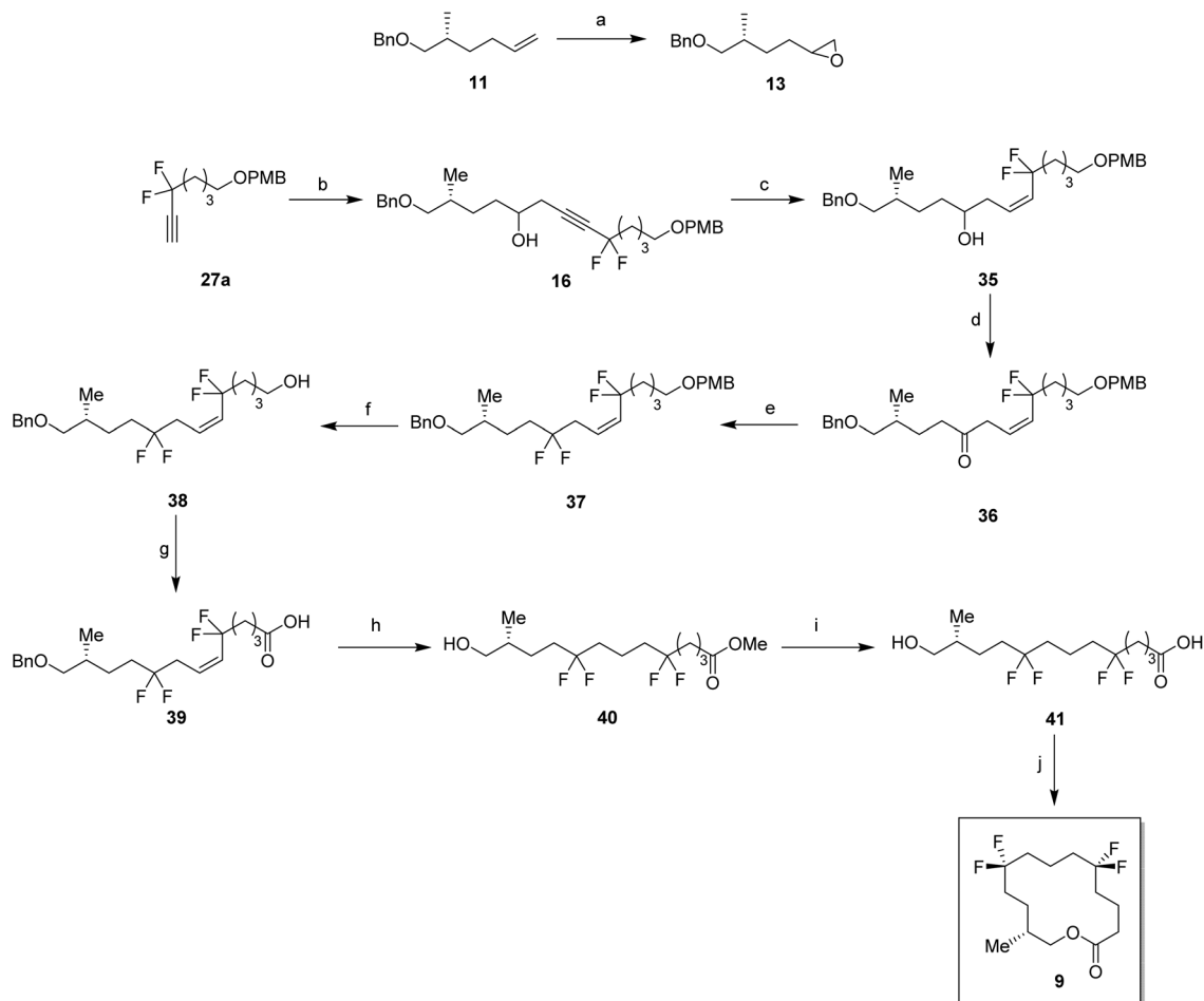
Scheme 5 Synthesis of musk lactone 9. Reagents and conditions: (a) m CPBA, DCM, r.t., 18 h, 55%; (b) (i) n BuLi, THF, −78 °C, 15 min. (ii) BF 3 ·OEt 2 , 15 min. (iii) Epoxide 13, THF, −78 °C–r.t., 20 h, 60%; (c) palladium (5% on barium sulfate), quinoline, pyridine, H 2 (1 atm), 22 h, 82% (d) DMP, DCM, r.t., 2 h, 57%; (e) DAST, 50 °C, 18 h, 27%; (f) DDQ, DCM, H 2 O, r.t., 2 h, 70%; (g) BAIB, TEMPO, CH 3 CN, H 2 O, r.t., 18 h, 49%; (h) palladium on carbon (10 wt%), H 2 , MeOH, r.t., 18 h, 59%; (i) LiOH, THF, H 2 O, r.t., 3 h, 70%; (j) 2,4,6-Trichlorobenzoyl chloride, NEt 3 , THF, r.t., 2.5 h. (ii) 4-DMAP, toluene, r.t., 3.5 h, 52%.
