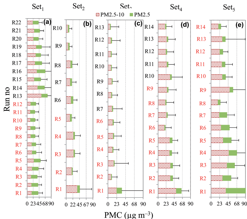
Fig. 2 In-cabin PMCs (PM 2.5-10 and PM 2.5 ) in two different fractions during (a) Set 1 , (b) Set 2 , (c) Set 3 , (d) Set 4 and (e) Set 5 . Please note that runs taken during morning hours are marked in red colour. For the sake of clarity only positive standard deviations are shown.
