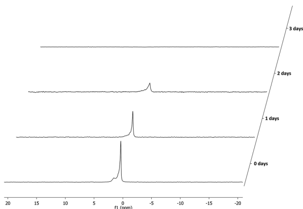
Fig. 3 Hydrolysis of representative supported phosphine-borane sulfate 3a-BH 3 monitored by 7 Li NMR spectroscopy.
