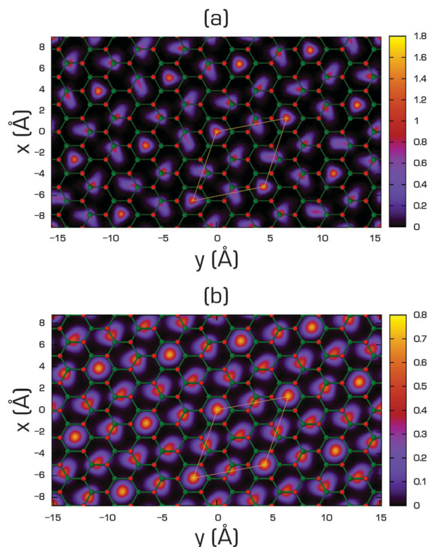
Fig. 14 Helium density (in \text{\AA}^{-2} ) on the x–y plane of the 2/7 phase of ^4\text{He} on fluorographene (a) and on graphane (b) compared with the geometry of the substrate. Small red balls are centred on the position of fluorine/hydrogen atoms and the small green ones on the carbon atoms. Thin white lines enclose the unit cell of the commensurate 2/7 phase [reprinted with permission from ref. 305. Copyright 2012 by the American Physical Society].
