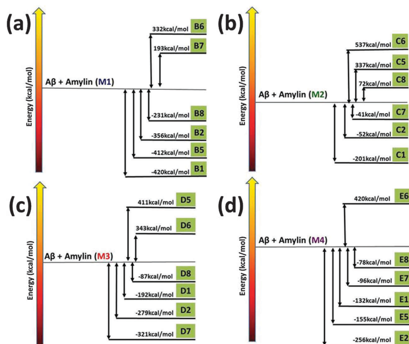
Fig. 3 The relative conformational energies of separated Aβ 1-42 hexamers and Amylin 1-37 hexamers (M1-M4) and Aβ 1-42 -Amylin 1-37 dodecamers.
