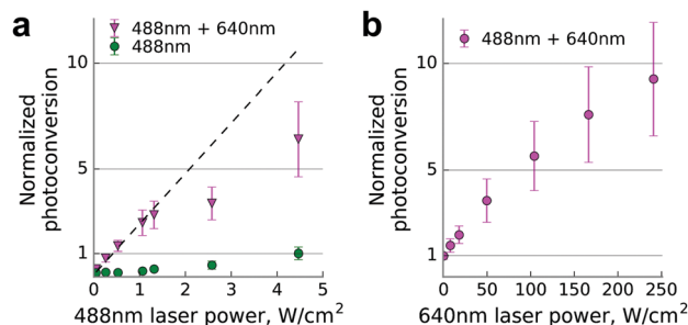
Fig. 2 Dendra2-actin photoconversion in live HeLa Kyoto cells in a wide field regime. (a) Photoconversion efficiency scaling at constant power of the 640 nm laser (240 W cm -2 ), normalized to the one achievable at the maximum power of the 488 nm laser (4.5 W cm -2 ). The dashed line shows a linear regression of the first three data points. For any given power (488 nm) value, data points differ significantly from the corresponding 488 nm + 640 nm ones (two-tailed unequal variance t -test, P < 0.001). (b) Photoconversion efficiency scaling at constant power of the 488 nm laser, set to the value just below the saturation point (1 W cm -2 ), normalized to the data point without 640 nm illumination. Data are mean \pm s.d. (error bars) for n = 23 cells.
