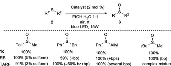
Scheme 3 Comparative study of catalyst 1c with Rose Bengal (RB) and tetra- O -acetylriboflavine (TARG) (bp = byproducts, bz = benzaldehyde) (see the ESI† for spectra).
