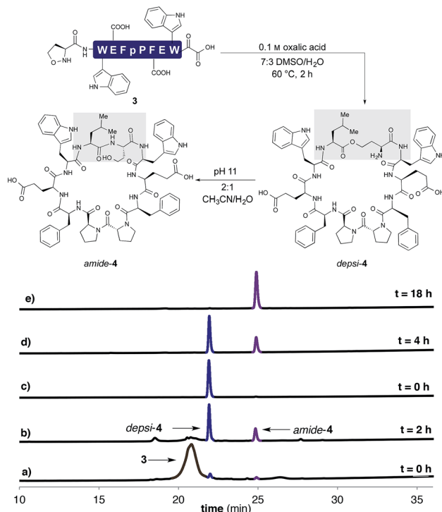
Scheme 2 Cyclization of 3 in 7 : 3 \text{DMSO}/\text{H}_2\text{O} with 0.1 M oxalic acid at 60 °C after (a) 0 h (b) 2 h. (c) Purified depsi-4 . (d) O,N -Acyl shift of depsi-4 at pH 11 in 2 : 1 \text{CH}_3\text{CN}/\text{H}_2\text{O} (200 mM phosphate buffer) after 4 h and (e) after 18 h.
