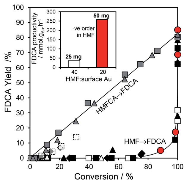
Fig. 5 (main) Disparate evolution of FDCA yield as a function of either HMF or HMFCa conversion over 25 mg \Delta ( \Delta ) 0.5 wt%, \blacklozenge ( \blacklozenge ) 1 wt%, \square ( \square ) 2 wt%, \blacksquare ( \blacksquare ) 5 wt%, and \blacktriangle ( \blacktriangle ) 10 wt% Au/HT catalysts, and 50 mg \bullet ( \bullet ) 2 wt% Au/HT; (inset) normalised FDCA productivity per Au atom as a function of HMF : surface Au molar ratio for 2 wt% Au/HT highlighting self-poisoning by high HMF concentrations.
