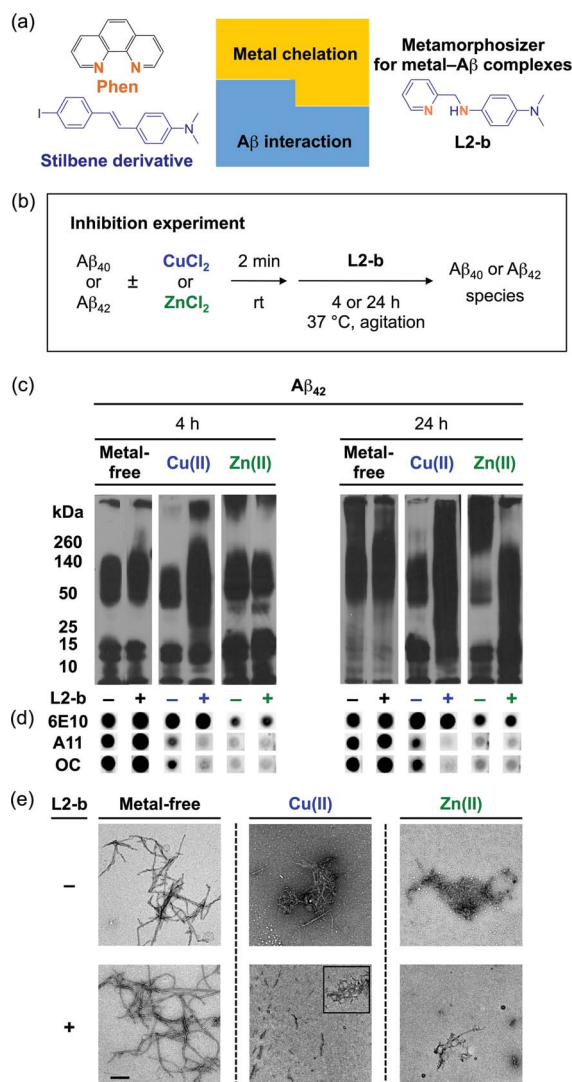
Fig. 1 Design principle of L2-b and its effect on metal-free and metal-induced A\beta aggregation. (a) Design principle of L2-b, a metamorphosizer for metal- A\beta complexes: a metal binding site (orange) is incorporated into an A\beta interacting framework (blue). (b) Scheme showing the inhibition experiment: metal-free or metal-treated [ CuCl_2 (blue) or ZnCl_2 (green)] A\beta_{40}/A\beta_{42} was incubated with (+) or without (–) L2-b for 4 h (left) and 24 h (right). Conditions: [ A\beta ] = 25 \mu M; [ Cu(II) or Zn(II) ] = 25 \mu M; [L2-b] = 50 \mu M; pH 6.6 (for Cu(II) samples) or pH 7.4 (for metal-free and Zn(II) samples); 37 °C; constant agitation. (c) Analysis of the size distribution of the resultant A\beta_{42} species by gel electrophoresis and Western blotting with an anti- A\beta antibody (6E10). (d) Dot blot analysis of the resulting A\beta_{42} species employing 6E10, an anti- A\beta oligomer antibody (A11), and an anti- A\beta fibril antibody (OC). (e) TEM images of the 24 h incubated samples (scale bar = 200 nm).
