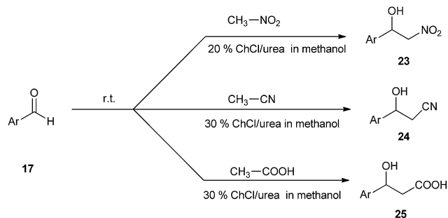
Scheme 9 Synthesis of nitroaldol using \text{ChCl}/\text{urea} .
