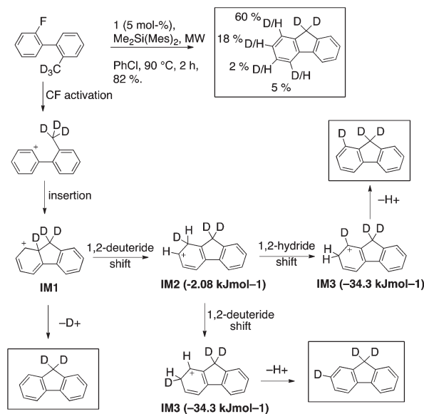
Scheme 4 Deuterium distribution in 3 produced from 2- d 3 ; postulated intermediates and their M06-2X/Def2-TZVP(chlorobenzene) computed energetics.
