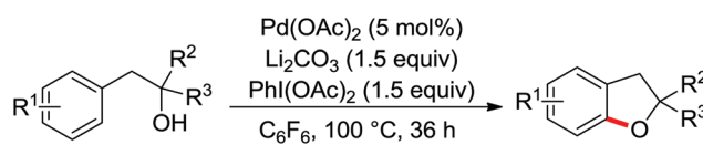
Scheme 354 Pd(II)-catalyzed hydroxyl-directed C–O cyclization.
