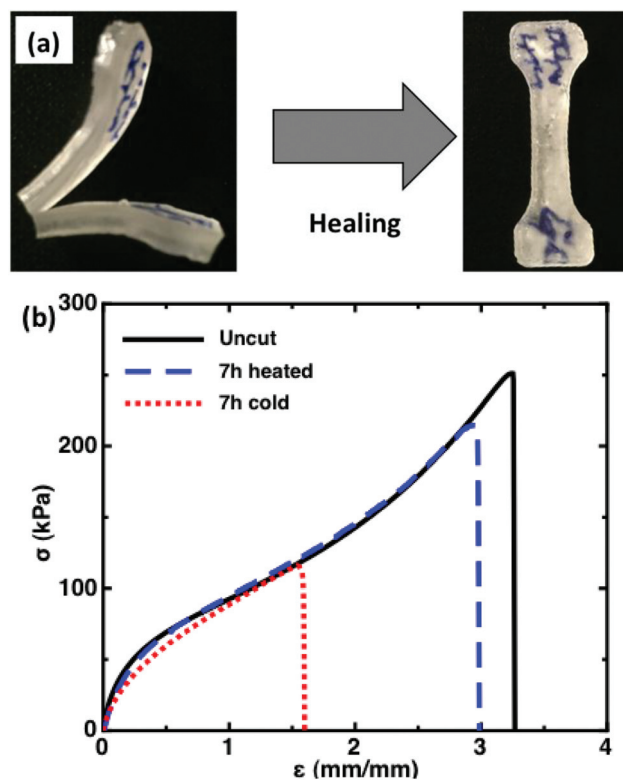
Fig. 1 (a) Left shows the PHEA-FMIDA-UPyA material directly after being cut with a razor. Right shows the same material with the scratch being much less prominent after 7 h of room temperature healing. (b) Comparison between the uncut and the PHEA-FMIDA-UPyA materials that were cut and healed under cold conditions for 7 h (room temperature) and cut and heated at 90\text{ }^\circ\text{C} for 7 h.
