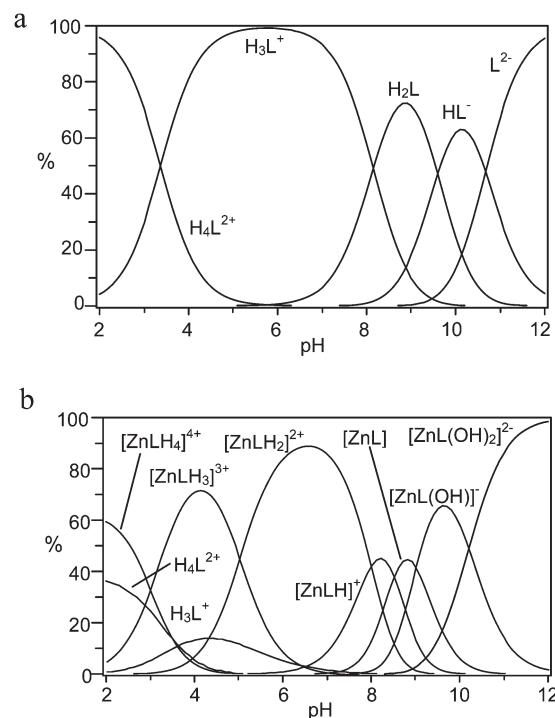
Fig. 1 Distribution diagrams of (a) the protonated species, and (b) the \text{Zn(II)} complexes formed by receptor 1 ( \text{L}^{2-} , \text{NMe}_4\text{Cl} , 0.1 M, 308 K).
