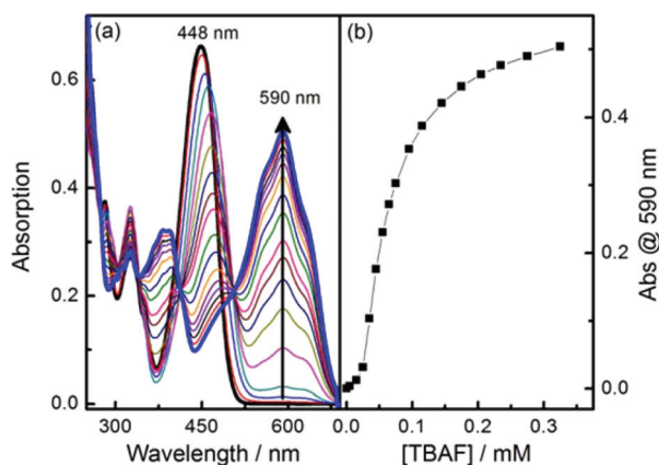
Fig. 2 (a) Absorption spectra changes of probe 1 along with addition of fluoride anion in MeCN; (b) Plot of absorption at 590 nm versus concentration of TBAF [ 1 ] = 10 \mu\text{M} .
