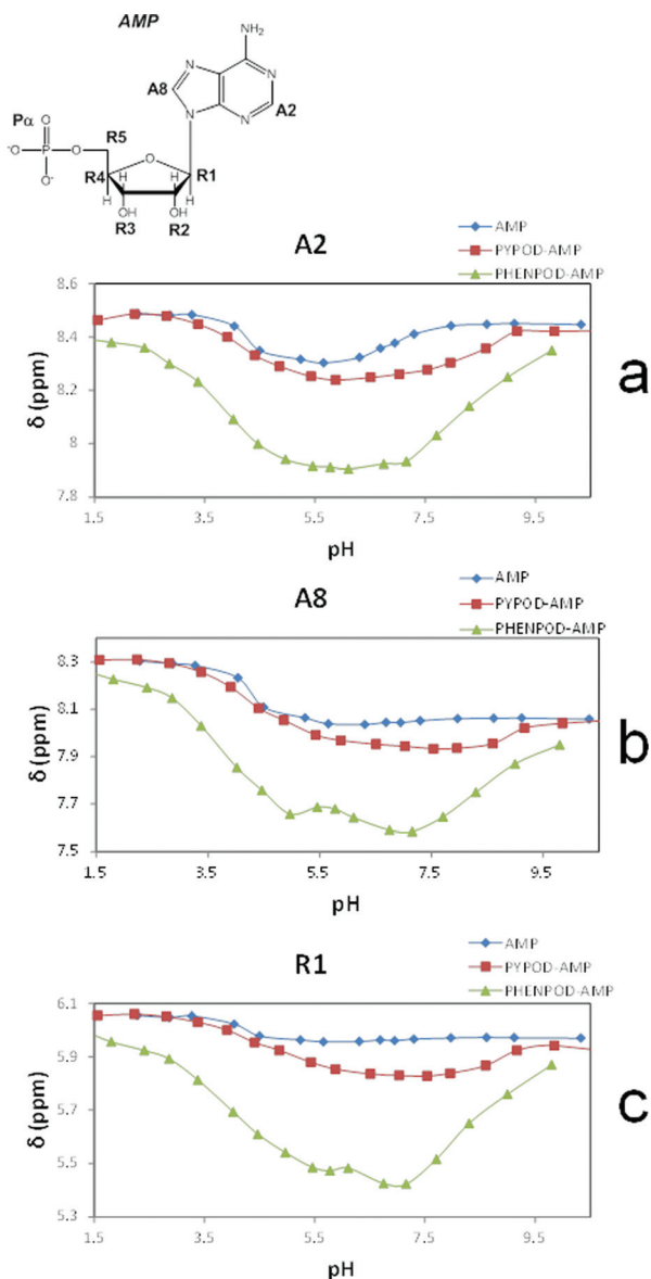
Fig. 5 Plot of ^1\text{H} NMR \delta (ppm) vs. pH of: AMP complexes with PYPOD and PHENPOD : aromatic protons (a) \text{H}_{\text{A}2} and (b) \text{H}_{\text{A}8} , anomeric signal (c) \text{H}_{\text{R}1} .
