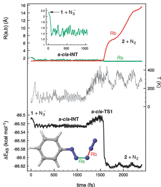
Fig. 3 Car-Parrinello Molecular Dynamics (CPMD) plots of the reaction between the diazonium cation 1 and the azide anion to yield phenyl azide 2 and dinitro.
