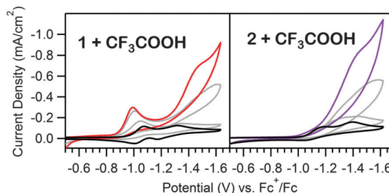
Fig. 3 Acid titrations of 0.5, 4, and 10 eq. of [CF_3COOH] into equimolar solutions of 1 and 2 ( 0.39\text{ mM} ). The black traces are the respective acid-free voltammograms. Voltammograms recorded at 100\text{ mV s}^{-1} in 100\text{ mM [Bu}_4\text{N][PF}_6\text{] CH}_3\text{CN} solutions.
