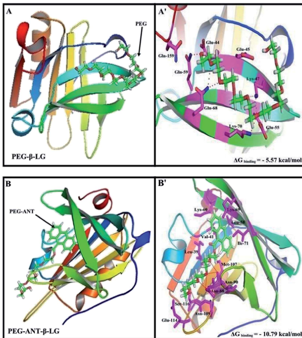
Fig. 7 Docking results of the PEG-β-LG and PEG-anthracene-β-LG complexes. View of the nearest amino acids surrounding PEG with H-bonding network and free binding energy.
