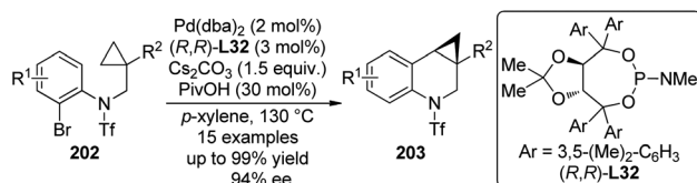
Scheme 60 The Pd-catalyzed asymmetric C–H bond functionalization reactions reported by Cramer.
