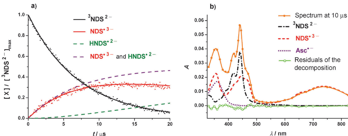
Fig. 3 Radical anion formation and decay in the quenching of ^3\text{NDS}^{2-} by \text{HAsc}^- under the conditions of Fig. 1a but with 2.65 mM of \text{HAsc}^- . (a) Measured and simulated concentration traces for species X, normalized to the initial triplet concentration. Black and red dots, experimental data points for the triplet and the radical anion; black solid line, fit of \exp[-k_1 t] to the triplet decay, best-fit parameter k_1 = 1.42 \times 10^5 \text{ s}^{-1} ; red solid line, fit of R(t) , R(t) = \eta \frac{k_1}{k_1 - k_2} (\exp[-k_2 t] - \exp[-k_1 t]) to the radical-anion curve with k_1 fixed at the previous value, best-fit parameters \eta = 0.56 and k_2 = 2.8 \times 10^4 \text{ s}^{-1} ; purple dashed line, calculated concentration S(t) of unprotonated plus protonated radical anion, i.e., S(t) = \eta(1 - \exp[-k_1 t]) ; dark green dashed line, calculated concentration trace for the protonated radical anion, i.e., difference between the two preceding curves. At 10 \mu\text{s} , the concentration ratio S(t)/R(t) , i.e., of the substrate-derived radicals in all their forms and in the form of the radical anion only, is 1.2 with the best-fit parameters given above. (b) Kinetic spectrum at 10 \mu\text{s} after the 308 nm pulse (orange solid line and filled dots); contributions of ^3\text{NDS}^{2-} (black dash-dotted line), \text{NDS}^{\bullet 3-} (red dashed line), and \text{Asc}^{\bullet -} (purple dotted line); residuals of the decomposition (light green solid line and open dots). Further explanation, see text.
