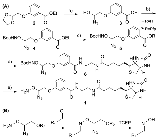
Scheme 1 (A) Synthesis of cleavable probe 1 (a) TMS-N 3 , SnCl 4 (b) (i) MsCl, Et 3 N, DCM (ii) BocNH 2 , DBU, Et 2 O (c) (i) NaOH, EtOH (ii) PfpTFA, Et 3 N, Et 2 O. (d) Biotin ethylenediamine, DMF (e) HCl:MeOH. (B) Reaction of 1 with the aldehyde moiety and subsequent cleavage to yield the oxime.
