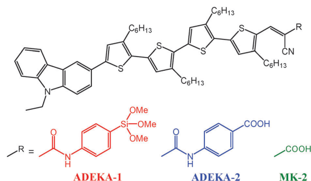
Fig. 1 Molecular structures of carbazole dyes with a trimethoxysilyl group (ADEKA-1) and with a carboxy group (ADEKA-2 and MK-2) as the anchor moiety for chemical bonding to the surface of the TiO 2 electrodes.
